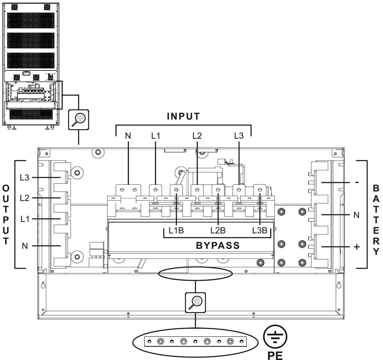
Abb. 9: Klemmenanschlüsse
