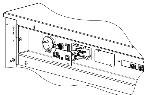
Abb. 11: Comm-Slot
